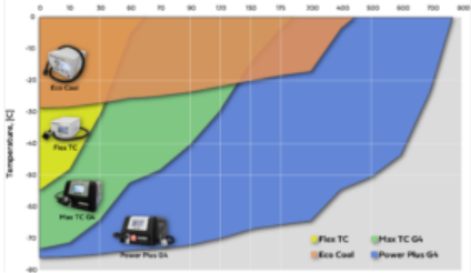
Cooling power of temperature forcing systems product line by Mechanical Devices
